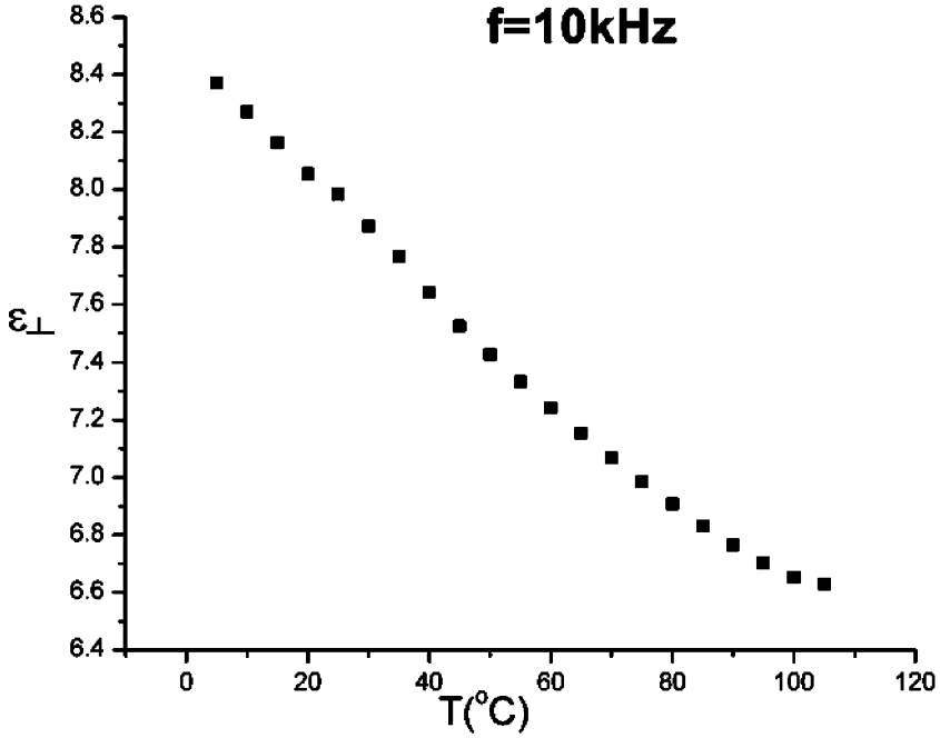
FIGURE 2 Dielectric permittivity \varepsilon_{\perp} vs. temperature (10°C to 105°C) at f = 10 kHz.
